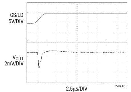
Midscale Glitch
