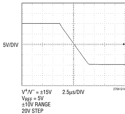
Negative Slew
