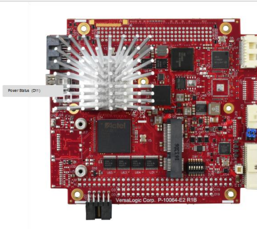
Figure 11. Location of the D11 Dual-color LED
