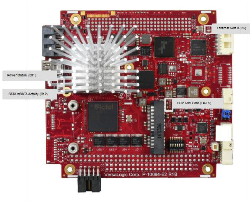
Figure 10. Locations of the LEDs/Indicators
