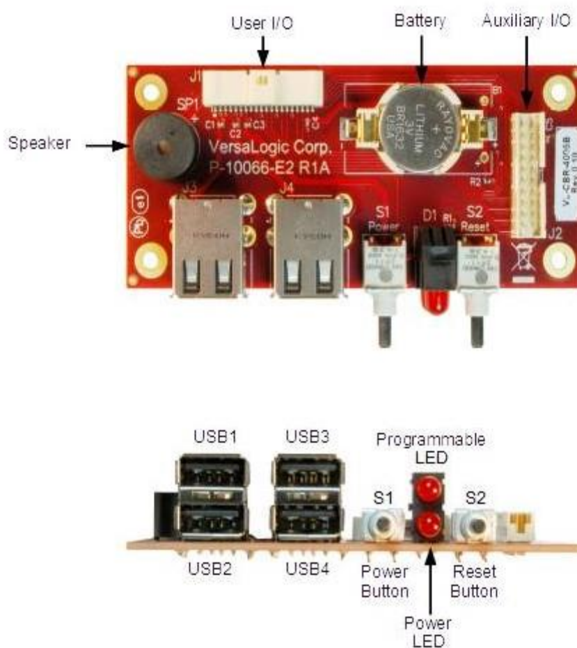
Figure 21. CBR-4005 Connectors, Switches, and LEDs
