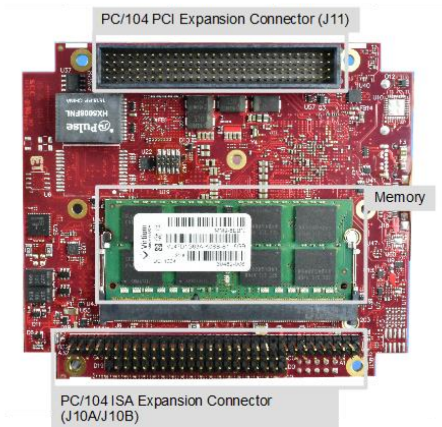
Figure 3. VL-EPM-39 Single Board Computer (Bottom Side)
