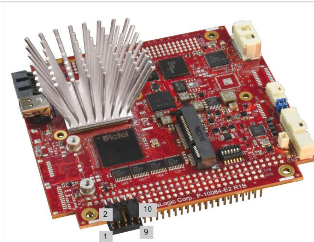
Figure 7. Location and Pin Orientation of the Main Power Connector
