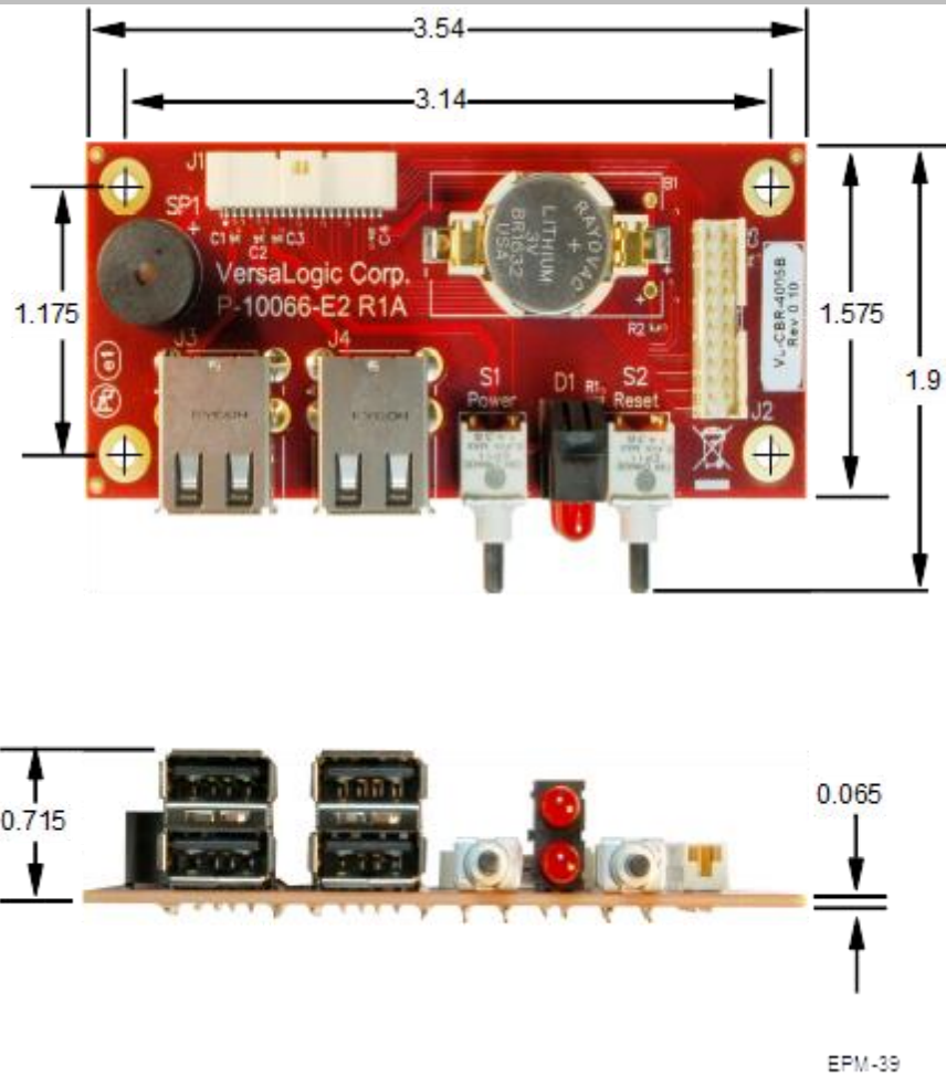
Figure 24. CBR-4005 Dimensions and Mounting Holes
