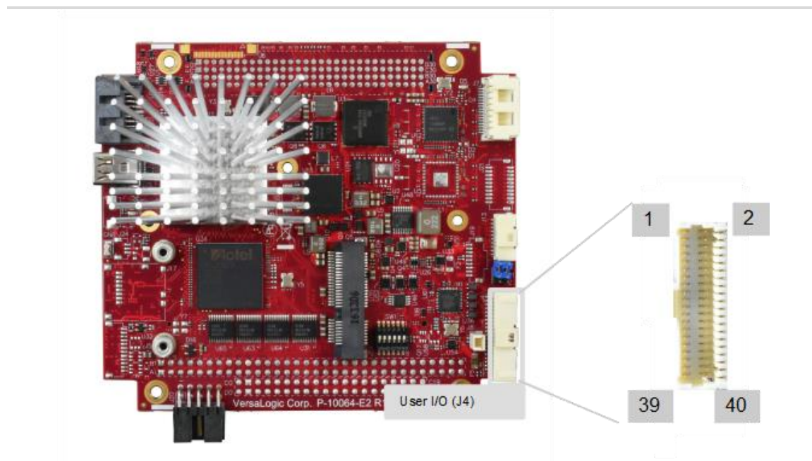
Figure 16. Location and Pin Orientation of User I/O Connector
