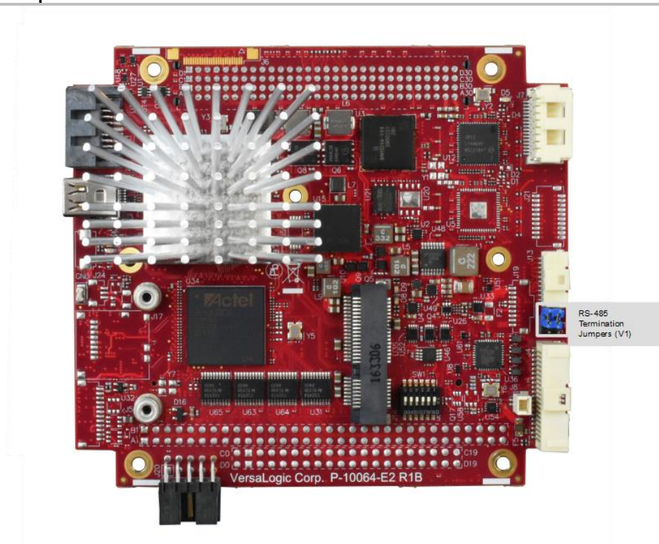
Figure 5. Jumper Block Locations
