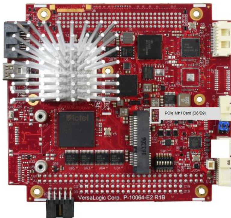
Figure 15. Location of PCIe Mini Card LEDs
