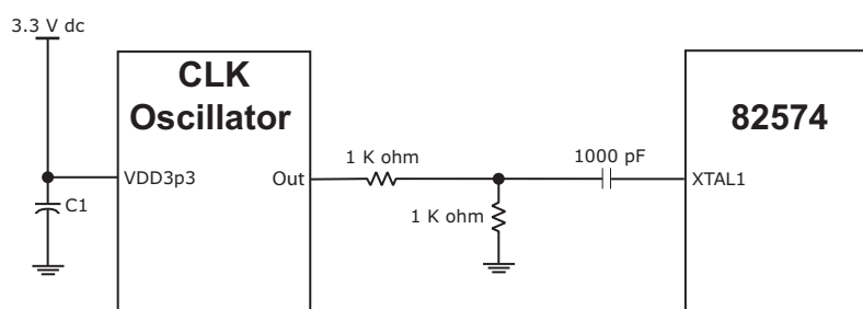
Figure 65. Oscillator Solution
