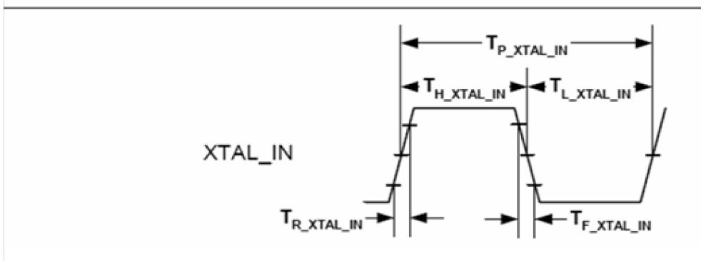
Figure 63. XTAL Timing Diagram
