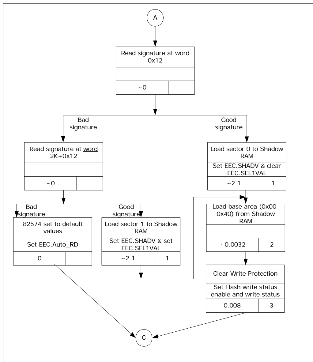
Figure 11. 82574 Initialization - Flash Load
