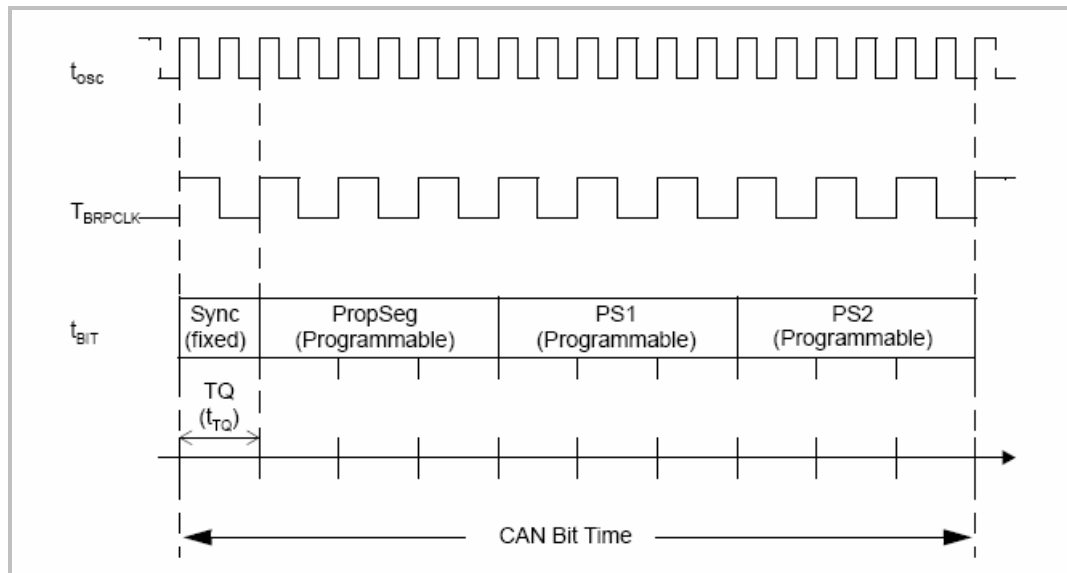
Figure 4. CANbus Bit
